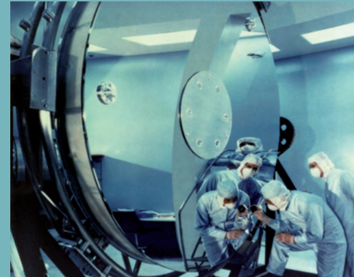
Figure 7.7. Hubble Space Telescope.
